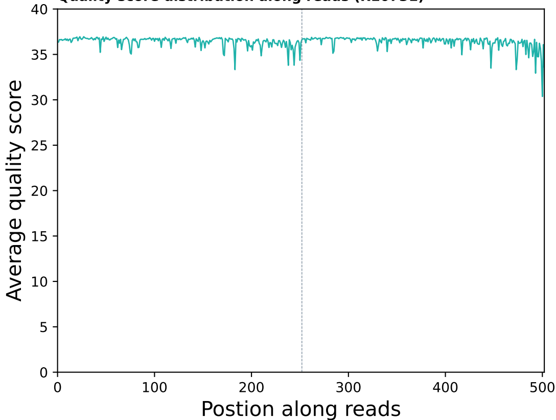
Quality score distribution along reads (R10731)
